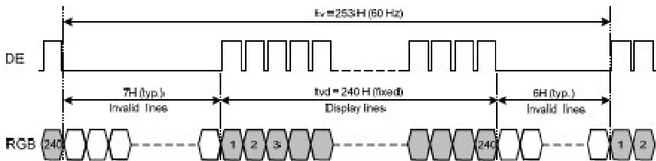
Fig. 9.2 Vertical Timing
