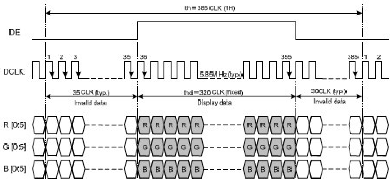
Fig. 9.1 Horizontal Timing
